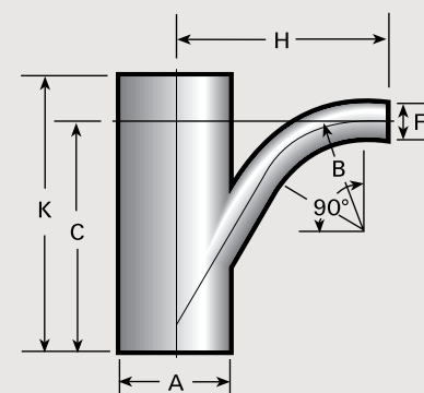
90° TY (straight ends)
